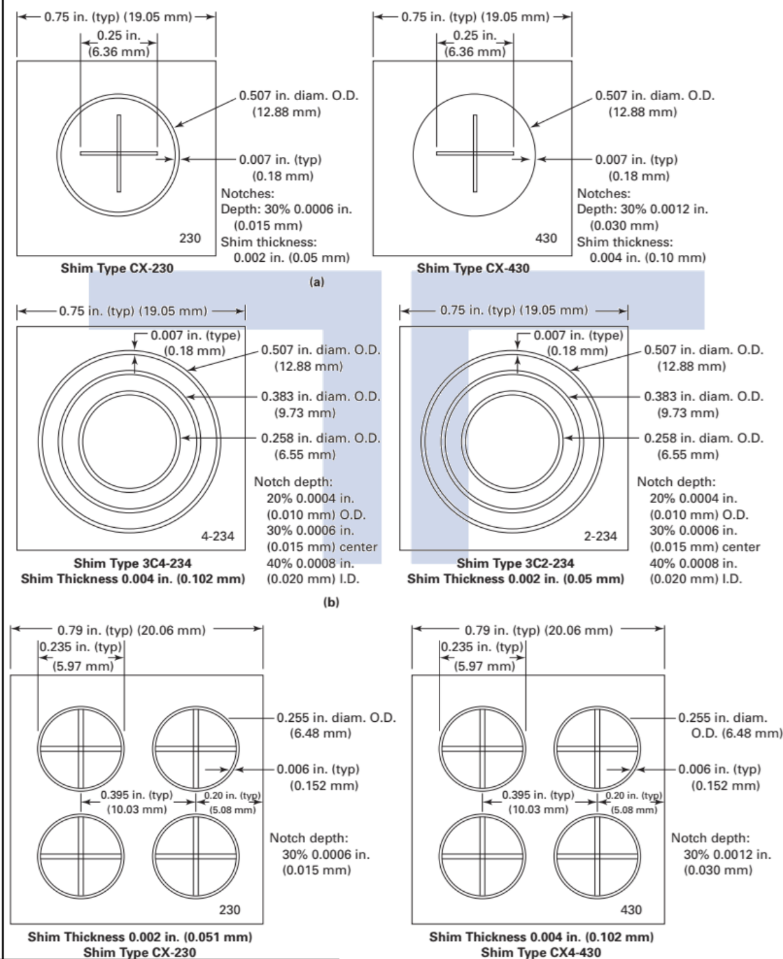
Figure T-764.2(b)(2) Artificial Flaw Shims
