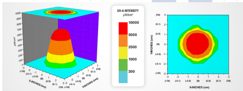
Surface Contour Profile at 15 in (38 cm)
