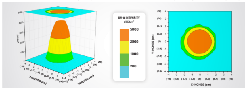
Surface Contour Profile at 15 in (38 cm)
